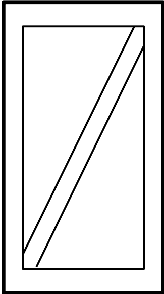
Global Pointer
