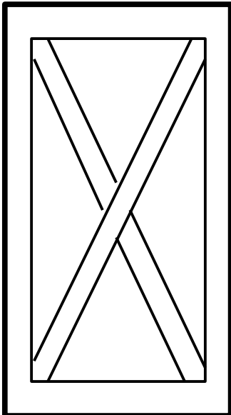
Global Pointer
